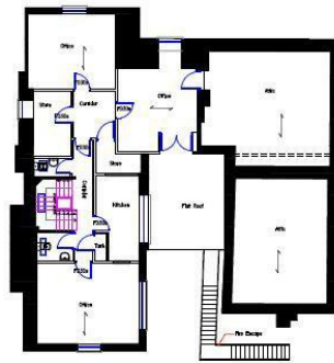
EXISTING SECOND FLOOR PLAN 1:100
